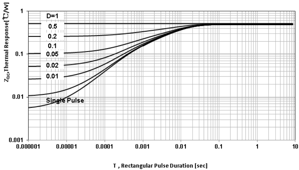
Figure 13 Maximum Effective Transient Thermal Impedance, Junction-to-Case
