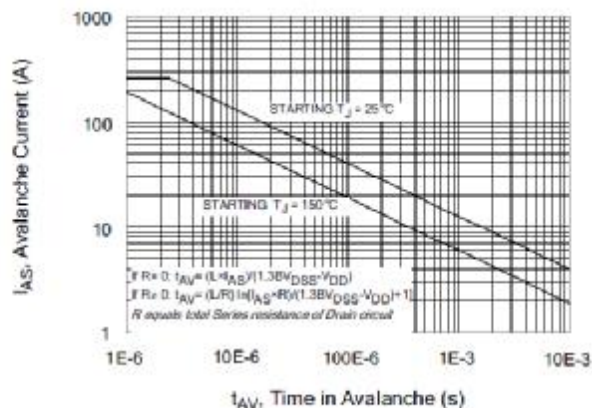
Figure 8. Undamped Inductive Switching Capability
