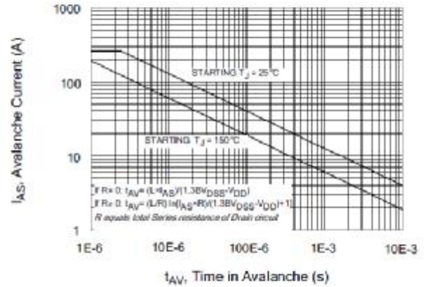
Figure 8. Undamped Inductive Switching Capability
