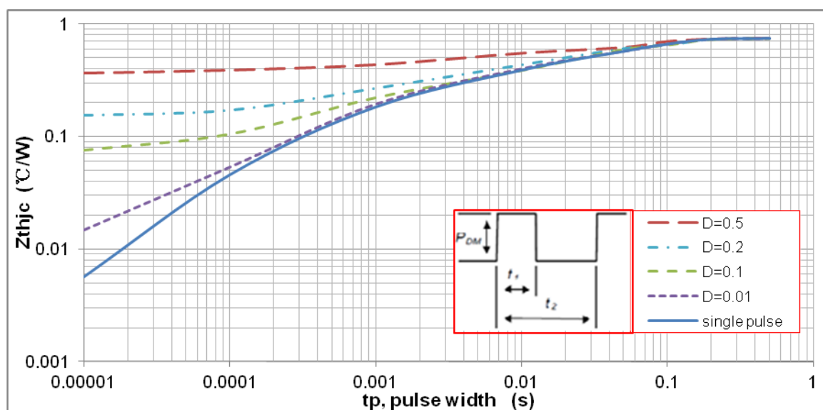
Figure19:normalised transient thermal impedance, junction-to-case
