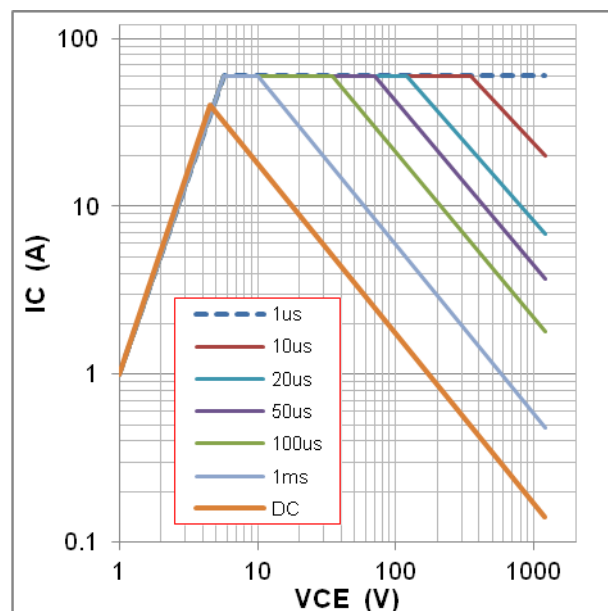
Figure4:forward SOA,TC=25°C,TJ≤150°C
