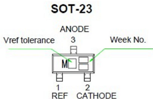
Pin Configuration
