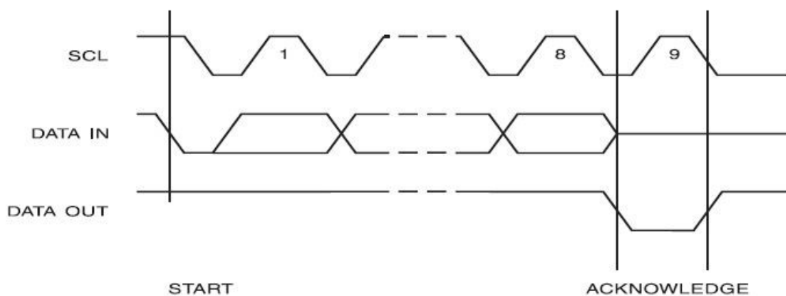
Figure 3. Output Acknowledge
