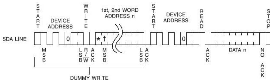
Figure 8. Random Read
