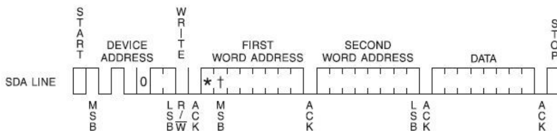
Figure 5. Byte Write
