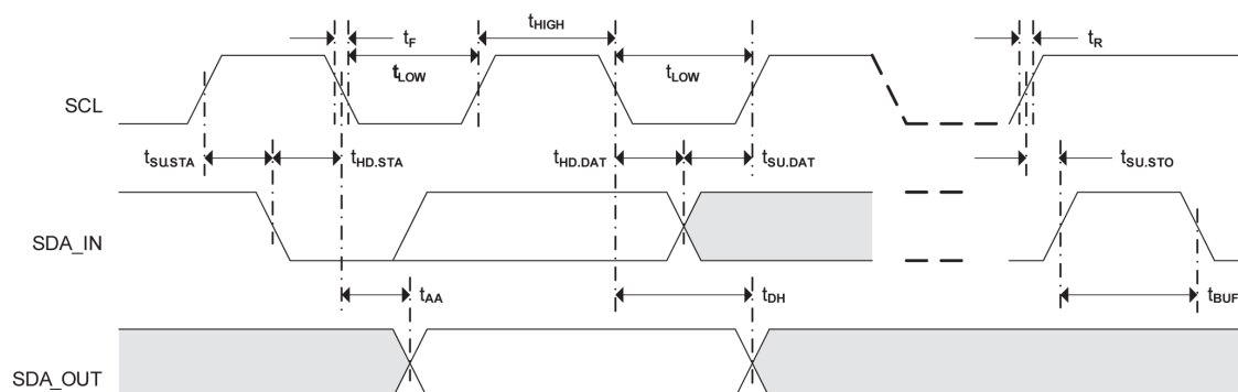
Figure 2. Bus Timing
