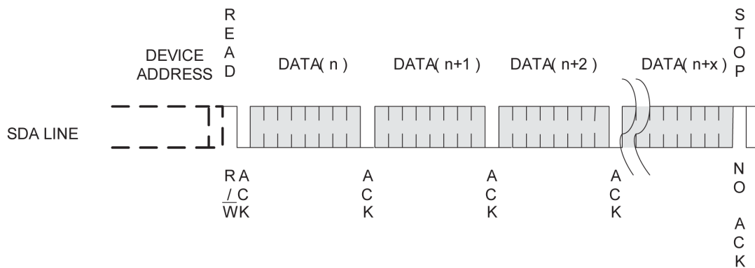
Figure 14. Sequential Read
