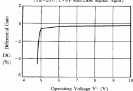
Differential Gain vs. Operating Voltage ( T_a = 25^\circ\text{C} , 1V_{P-P} staircase signal input)
