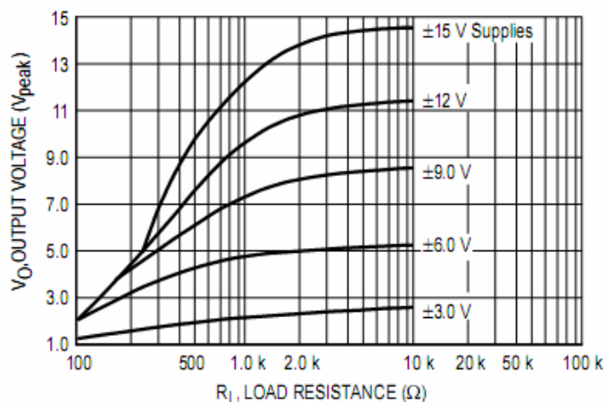
Figure 8. Positive Output Voltage Swing versus Load Resistance
