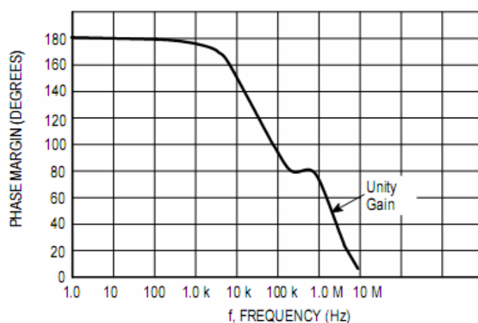
Figure 7. Phase Margin versus Frequency
