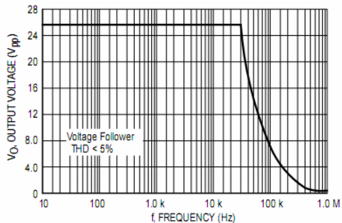
Figure 10. Power Bandwidth (Large Signal Swing versus Frequency)
