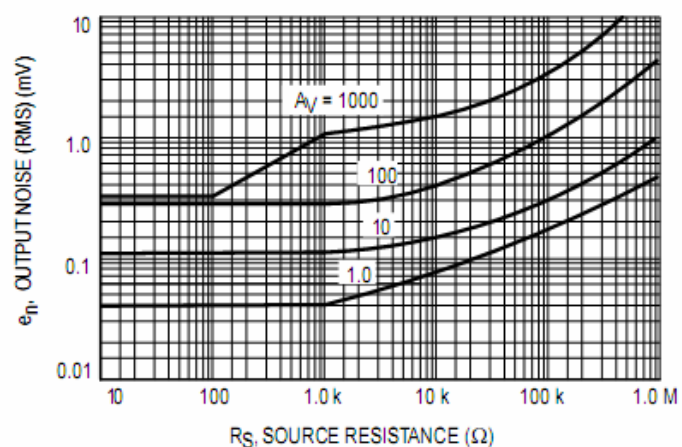
Figure 3. Output Noise versus Source Resistance
