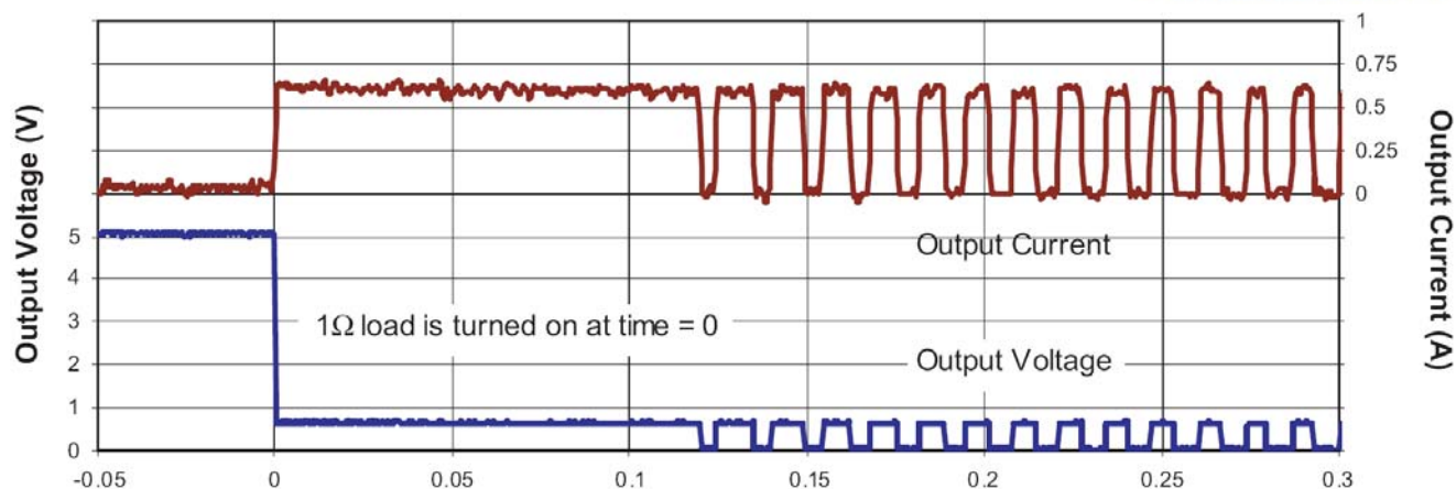
Figure 2: Overload Operation.
