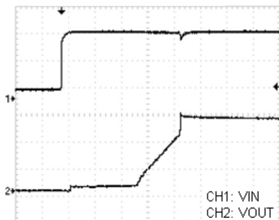
SW Waveform
