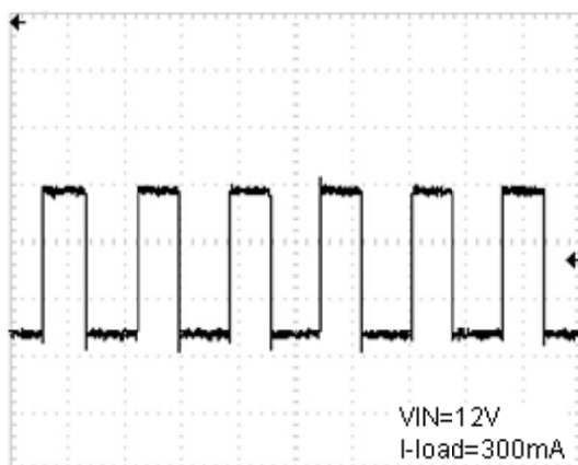
SW Waveform
