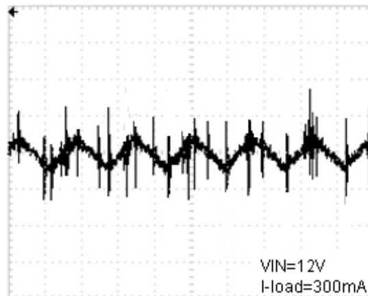
Output Waveform
