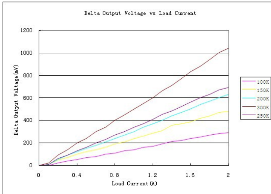
Figure 1. Delta Output Voltage vs Load Current
