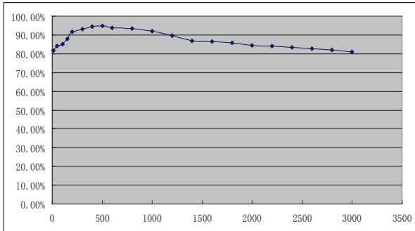
Vin=5V, Vout=1.8V
