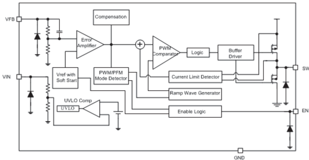
Figure 2. HM3430 Block Diagram
