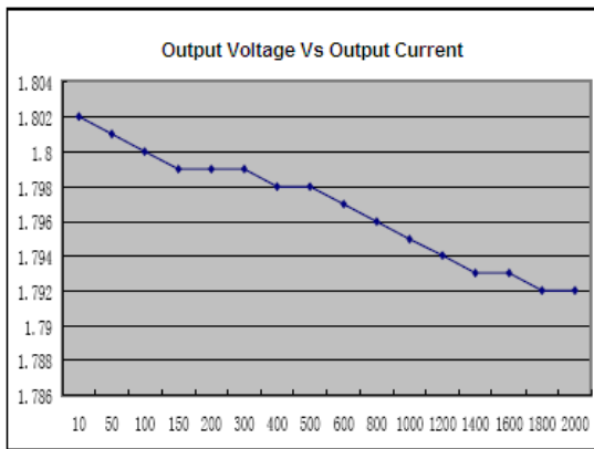
V_{in}=3.6V, V_{out}=1.8V
