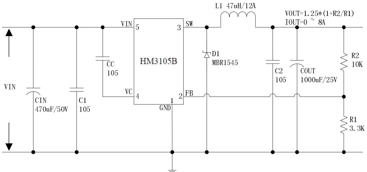
Figure4. HM3105B Typical Application Circuit (VIN=8V~40V, VOUT=5V/8A)
