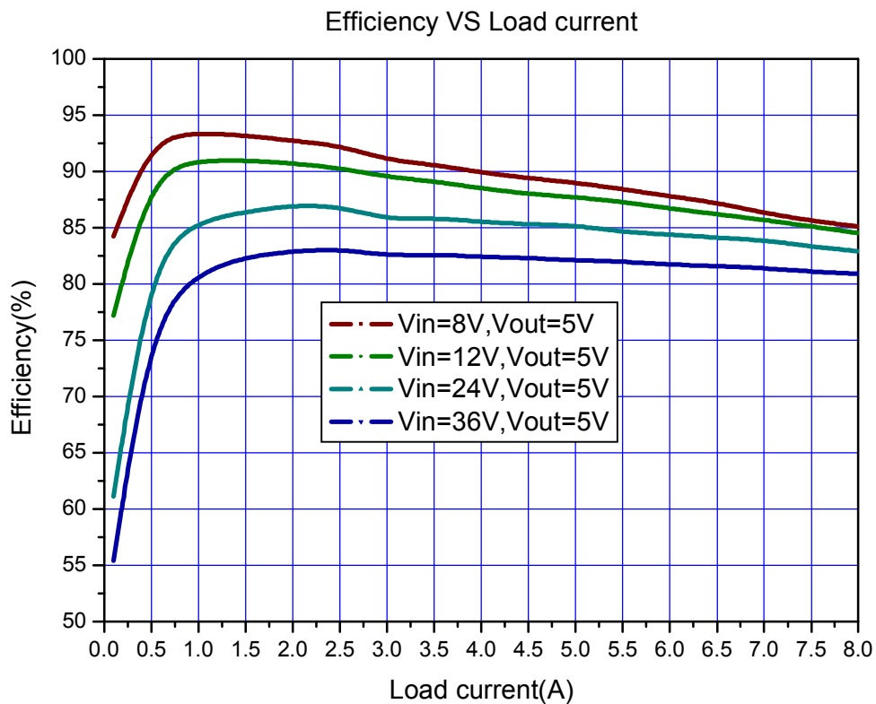
Figure6. HM3105B System Efficiency Curve
