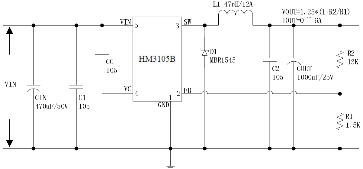
Figure7. HM3105B System Parameters Test Circuit (VIN=15V~40V, VOUT=12V/6A)
