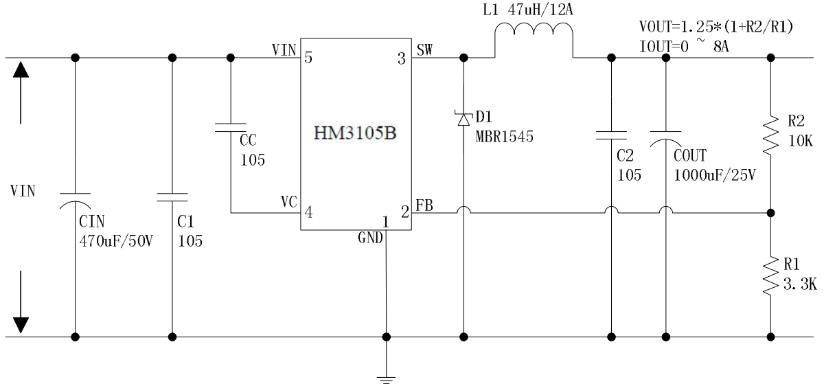
Figure5. HM3105B System Parameters Test Circuit (VIN=8V~40V, VOUT=5V/8A)
