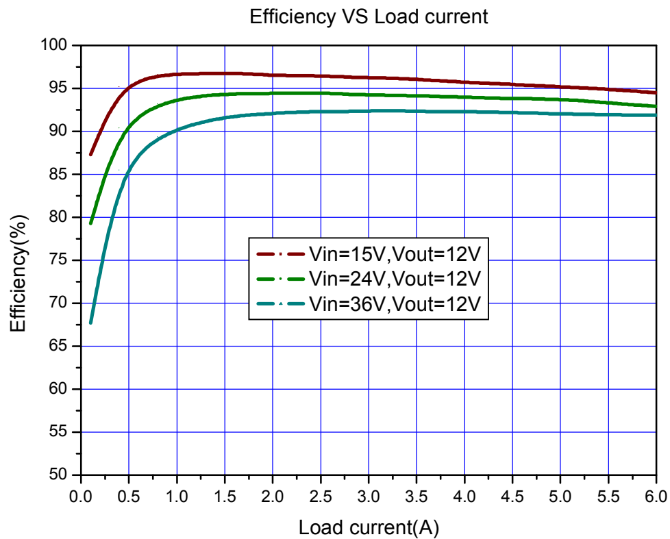
Figure8. HM3105B System Efficiency Curve
