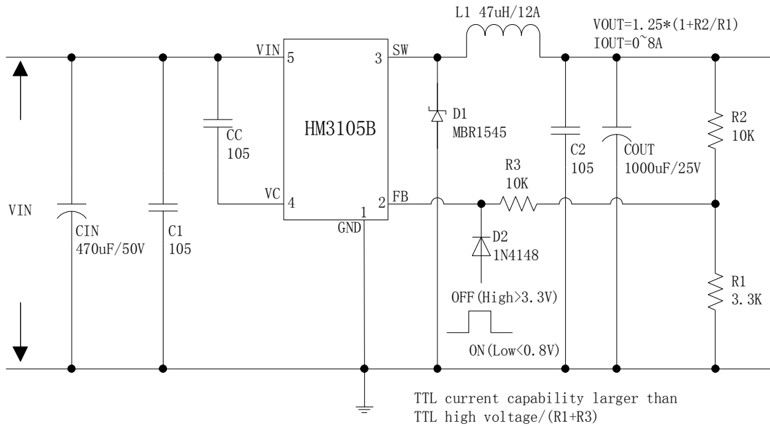
Figure9. HM3105B Typical Application Circuit
