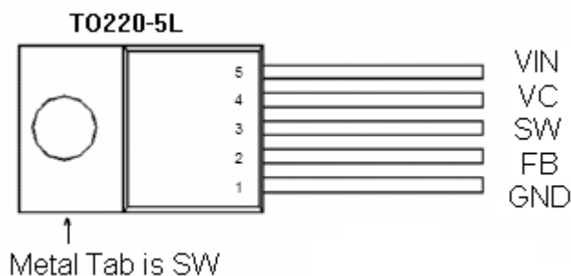
Figure2. Pin Configuration of HM3105B (Top View)
