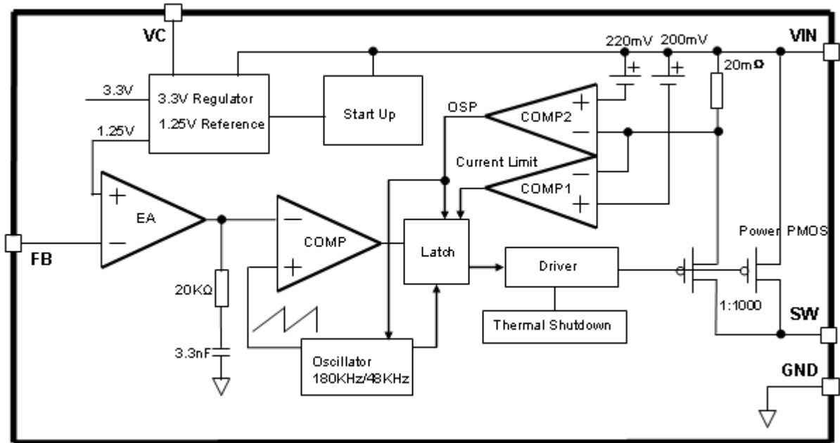
Figure3. Function Block Diagram of HM3105B
