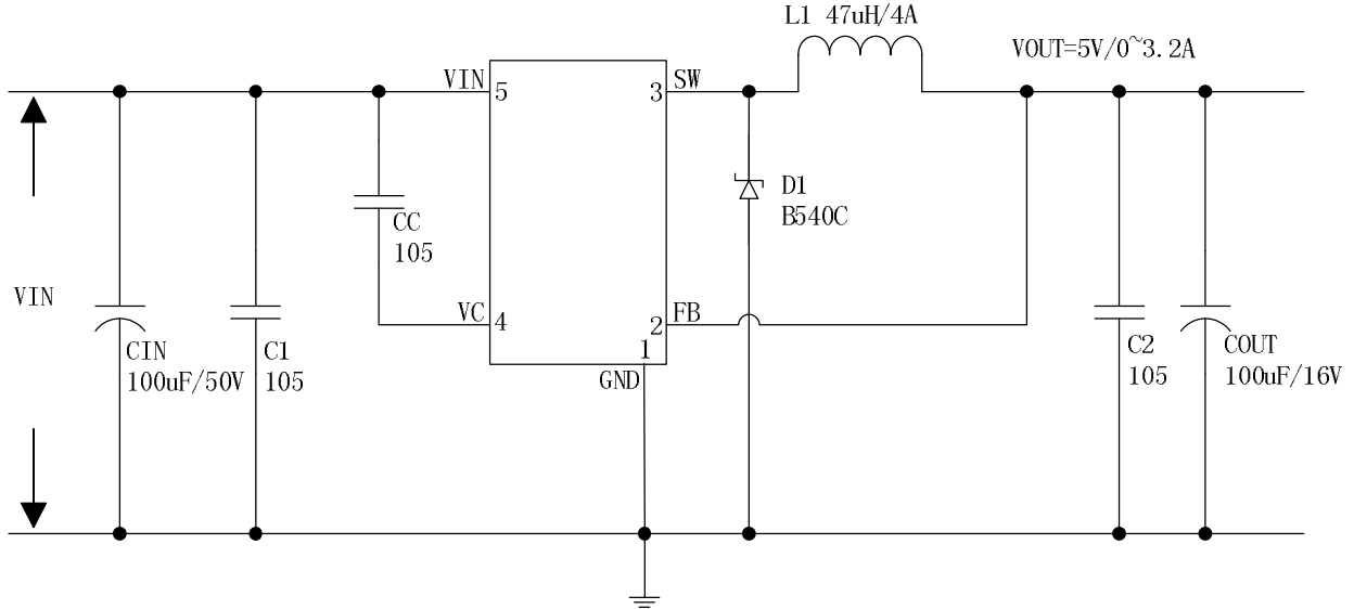
Figure5. HM3513 System Parameters Test Circuit (VIN=8V~40V, VOUT=5V/3.2A)
