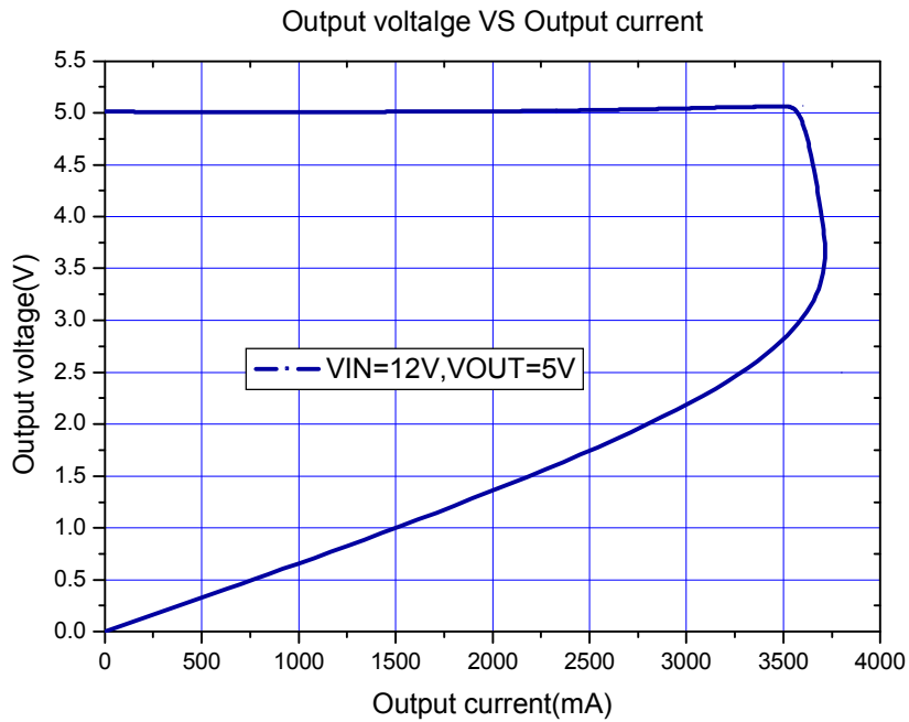
Figure6. HM3513 System Output Constant Current Curve
