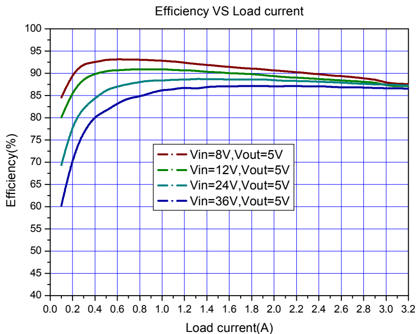
Figure7. HM3513 System Efficiency Curve
