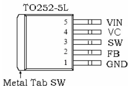
Figure2. Pin Configuration of HM3513 (Top View)
