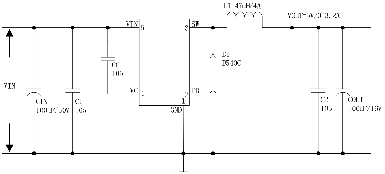
Figure4. HM3513 Typical Application Circuit (VIN=8V~40V, VOUT=5V/3.2A)
