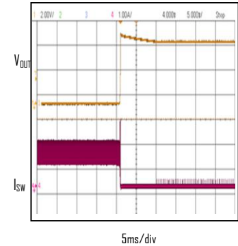
Short-Circuit Recovery V_{IN}=24\text{V}, V_{OUT}=5\text{V}, I_{OUT}=Short\text{ to }0\text{A}
