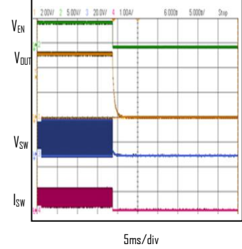
Shutdown Waveform with EN V_{IN}=30\text{V}, V_{OUT}=5\text{V}, I_{OUT}=0.5\text{A}
