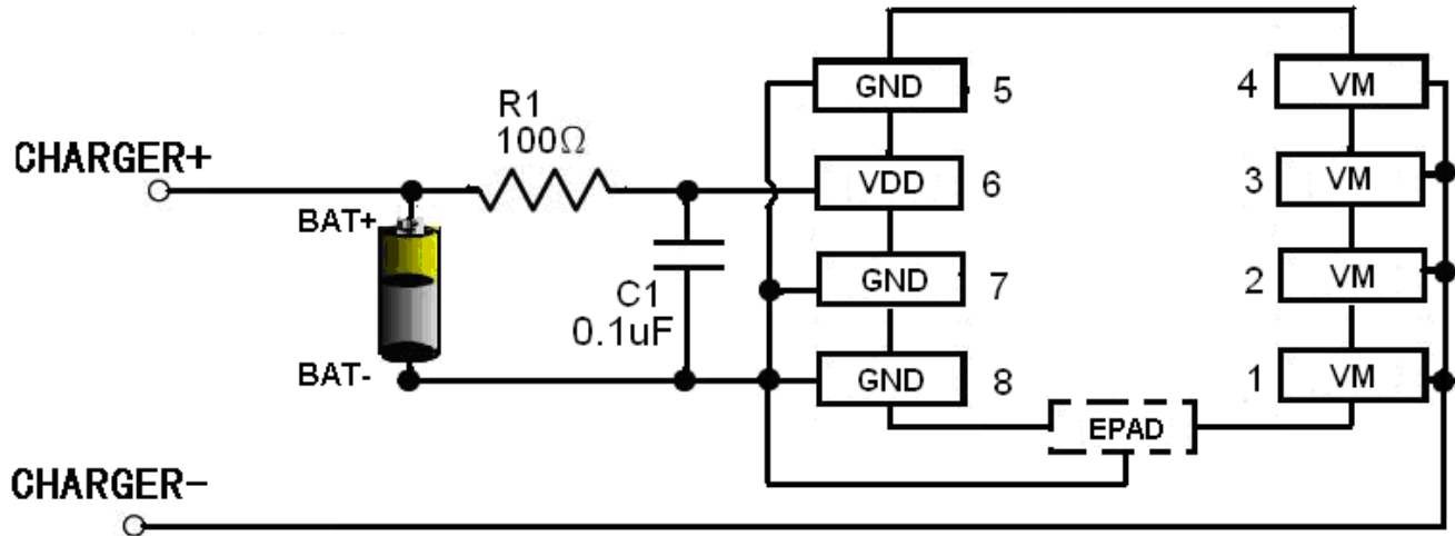
Fig 6 HM9905 in a Typical Battery Protection Circuit
