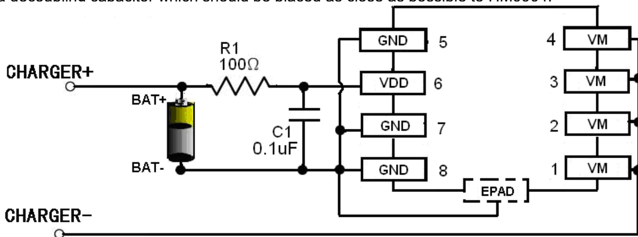
Fig 6 HM9904 in a Typical Battery Protection Circuit
