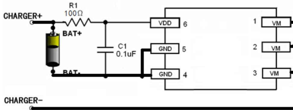
Fig 6 HM5469A in a Typical Battery Protection Circuit
