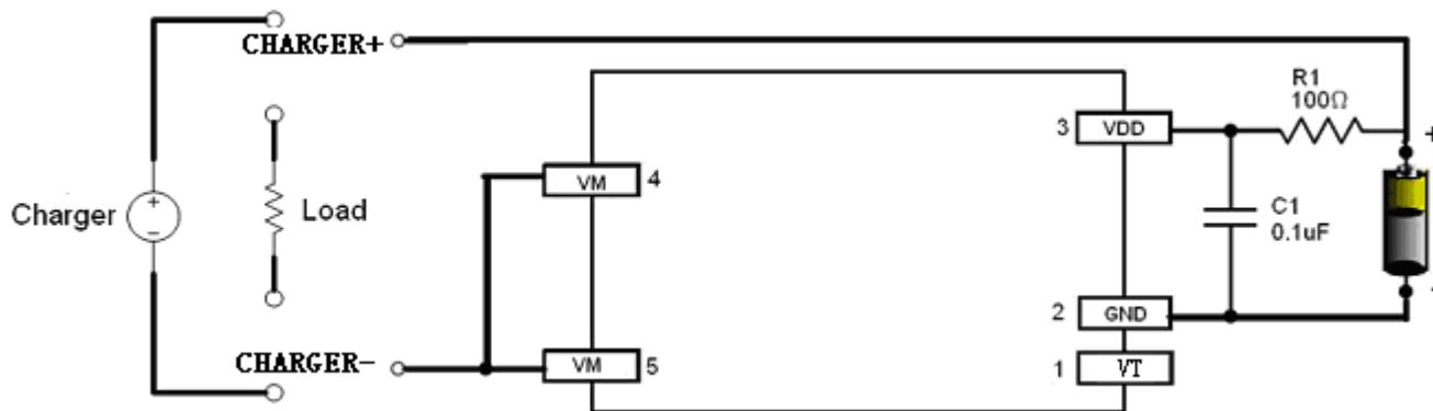
Fig 6 HM5453D in a Typical Battery Protection Circuit
