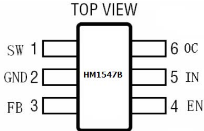
Figure 3. PIN Configuration
