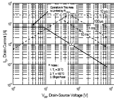
Figure 9-2. Maximum Safe Operating Area for HM7N80F
