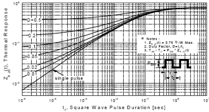
Figure 11-1. Transient Thermal Response Curve for HM7N80
