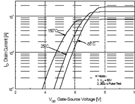
Figure 2. Transfer Characteristics
