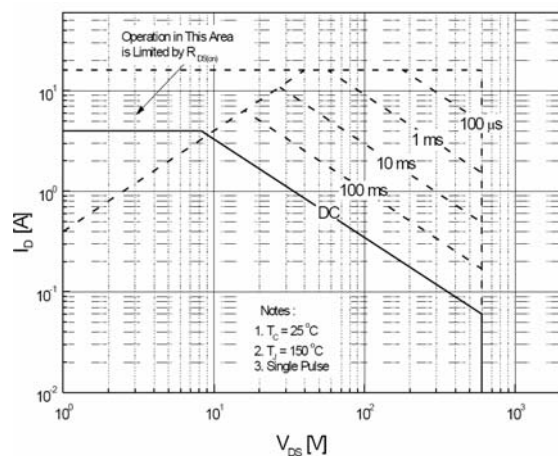
Maximum Safe Operating Area For HM4N60F
