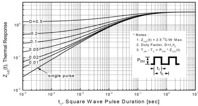
Transient Thermal Response Curve For HM4N60
