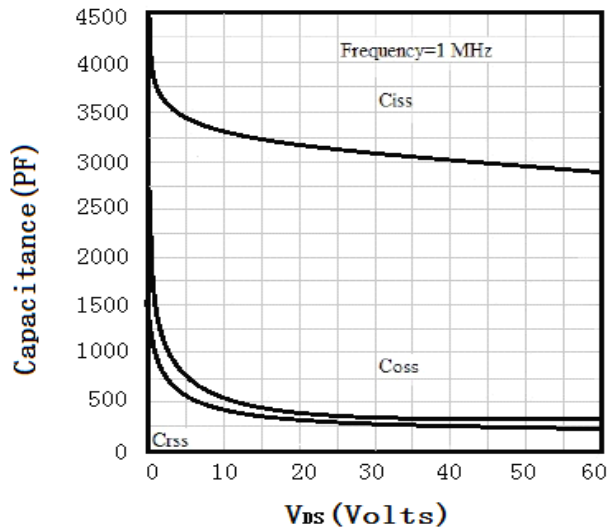
Figure10. Capacitance
