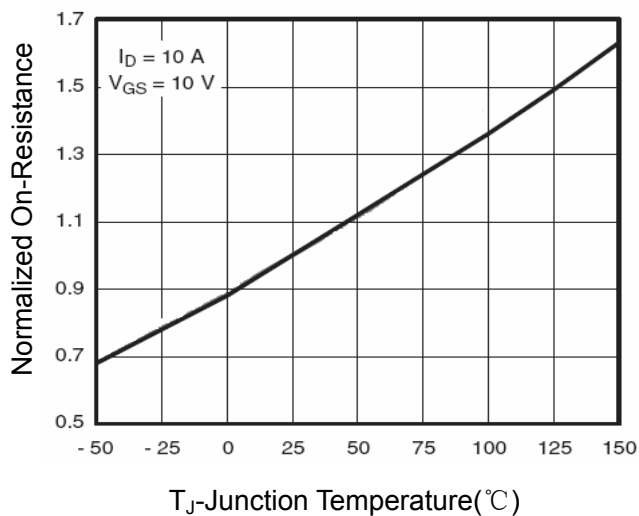
Figure 8 Drain-Source On-Resistance
