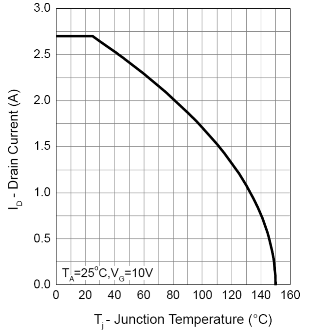
Drain Current
