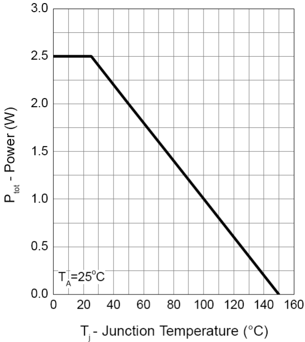
Power Dissipation
