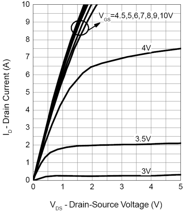
Output Characteristics
