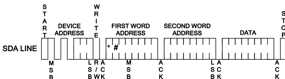
Figure 3: Byte Write
