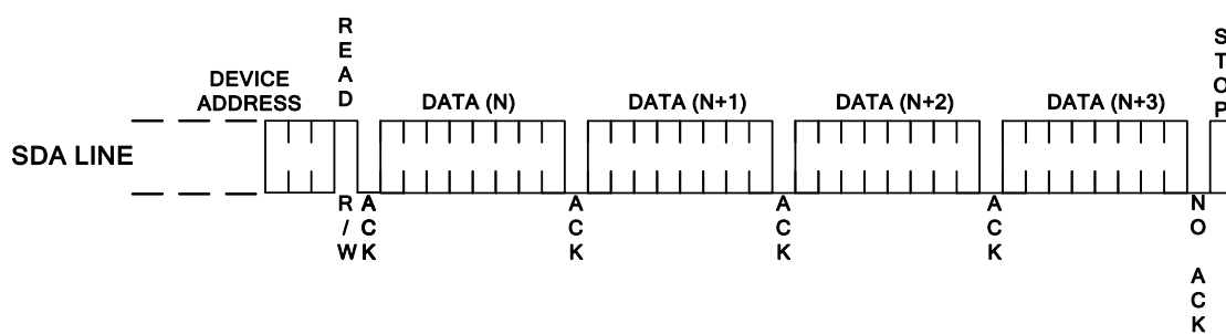
Figure 6: Sequential Read
