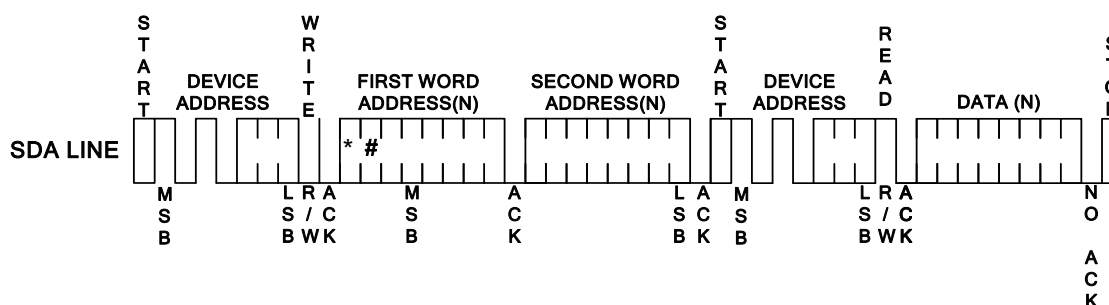
Figure 7: Random Read
