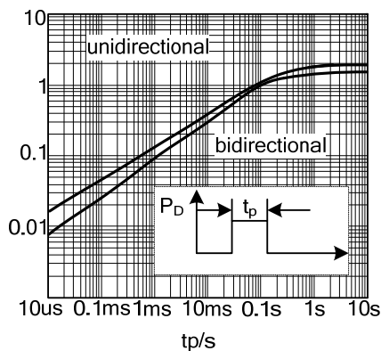
Transient Thermal Impedance Z_{th\ j-mb} , Vs Pulse Width, t_p
