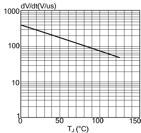
Typical, Critical rate of rise of off-state Voltage, dV_D/dt Versus Junction Temperature T_J
