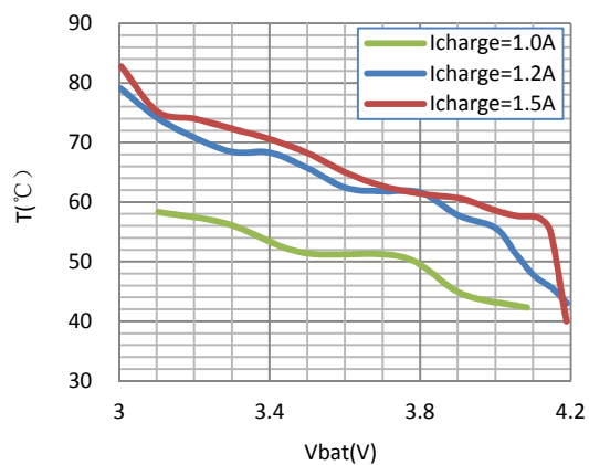
IC Temperature vs Battery Voltage
