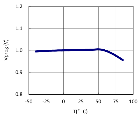
PROG Pin Voltage vs Temperature
