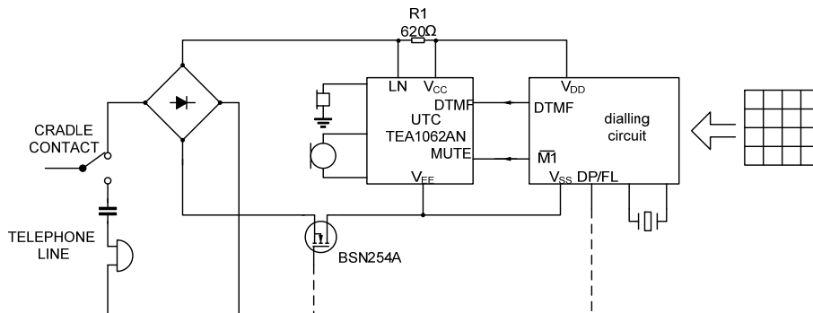
Fig.16 Typical applications of the UTC TEA1062N/TEA1062AN (simplified)
