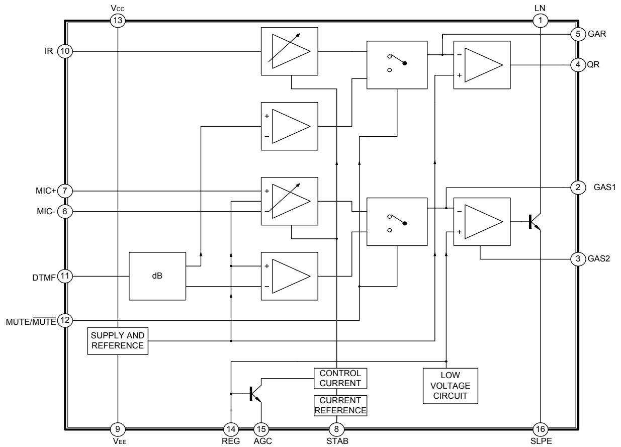
Fig. 2 Block Diagram
