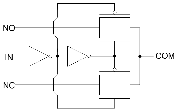
Logic Symbol
