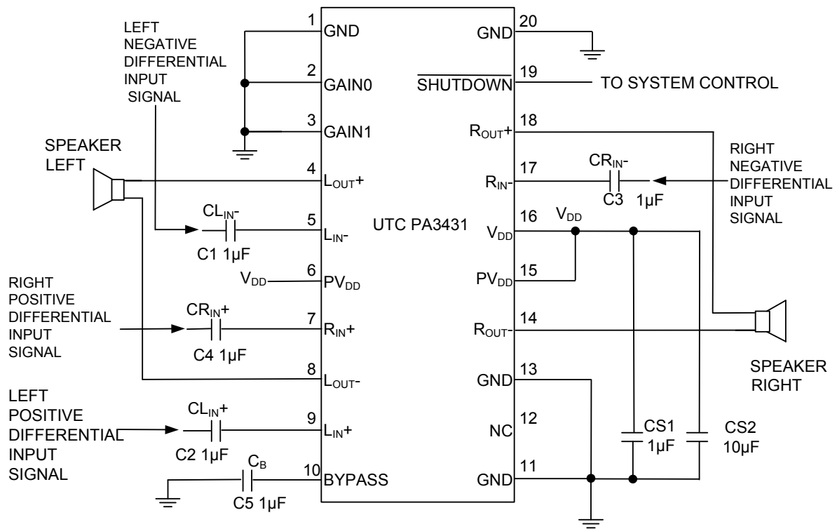
Typical Application Circuit Using Differential Inputs
