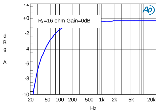
Frequency Response — SE
