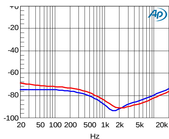
Cross-Talk—BTL
