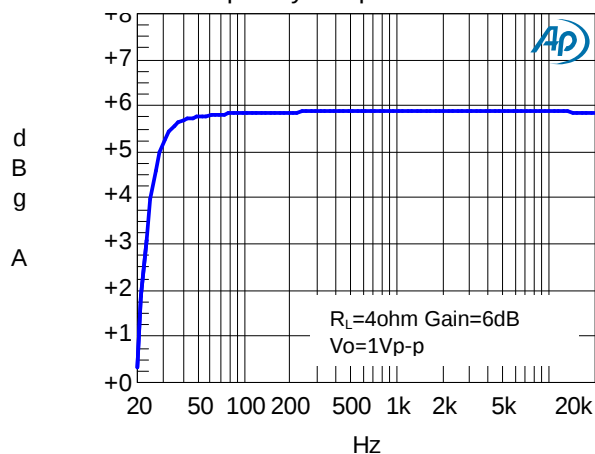
Frequency Response—BTL
