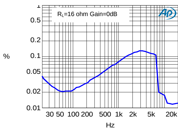
THD+N vs Frequency — SE
