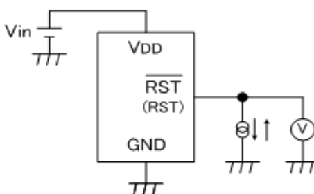
④-b open drain output type
