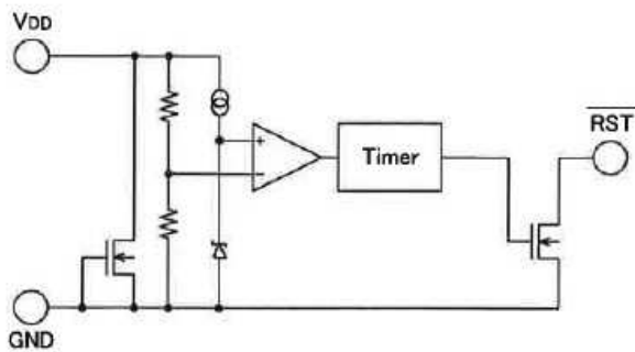
N channel open-drain
