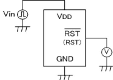
④-b open drain output type
