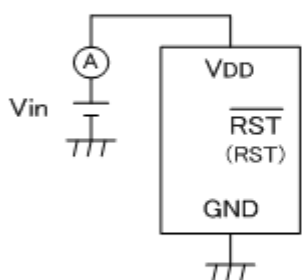
④-a CMOS output type
