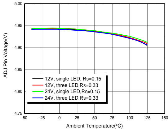
V ADJ Vs. Temperature L=47uH
