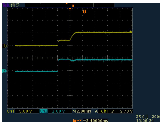
I_{out}=100mA
