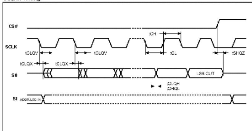
Output Timing
