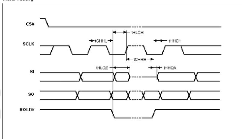
Hold Timing
