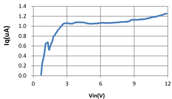
5. I_q ( V_{out}=2.8V )
