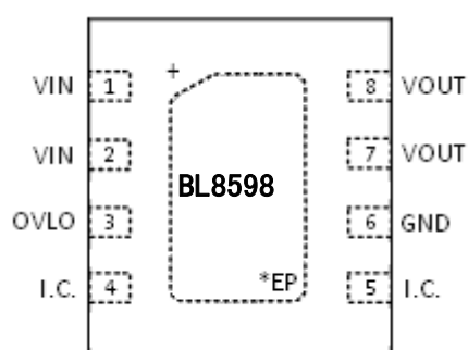
DFN2x2-8L
