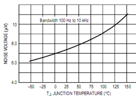
Figure 14. Output Noise
