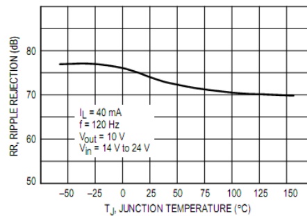
Figure 6. Ripple Rejection
