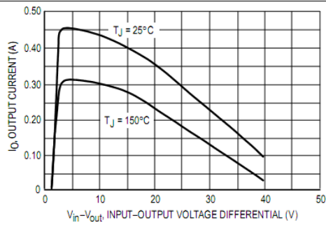
Figure 7. Current Limit
