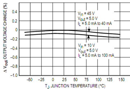
Figure 5. Load Regulation
