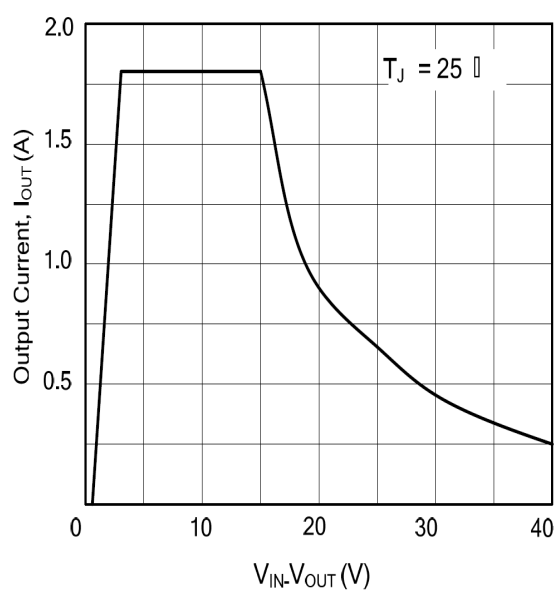
Current Limit
